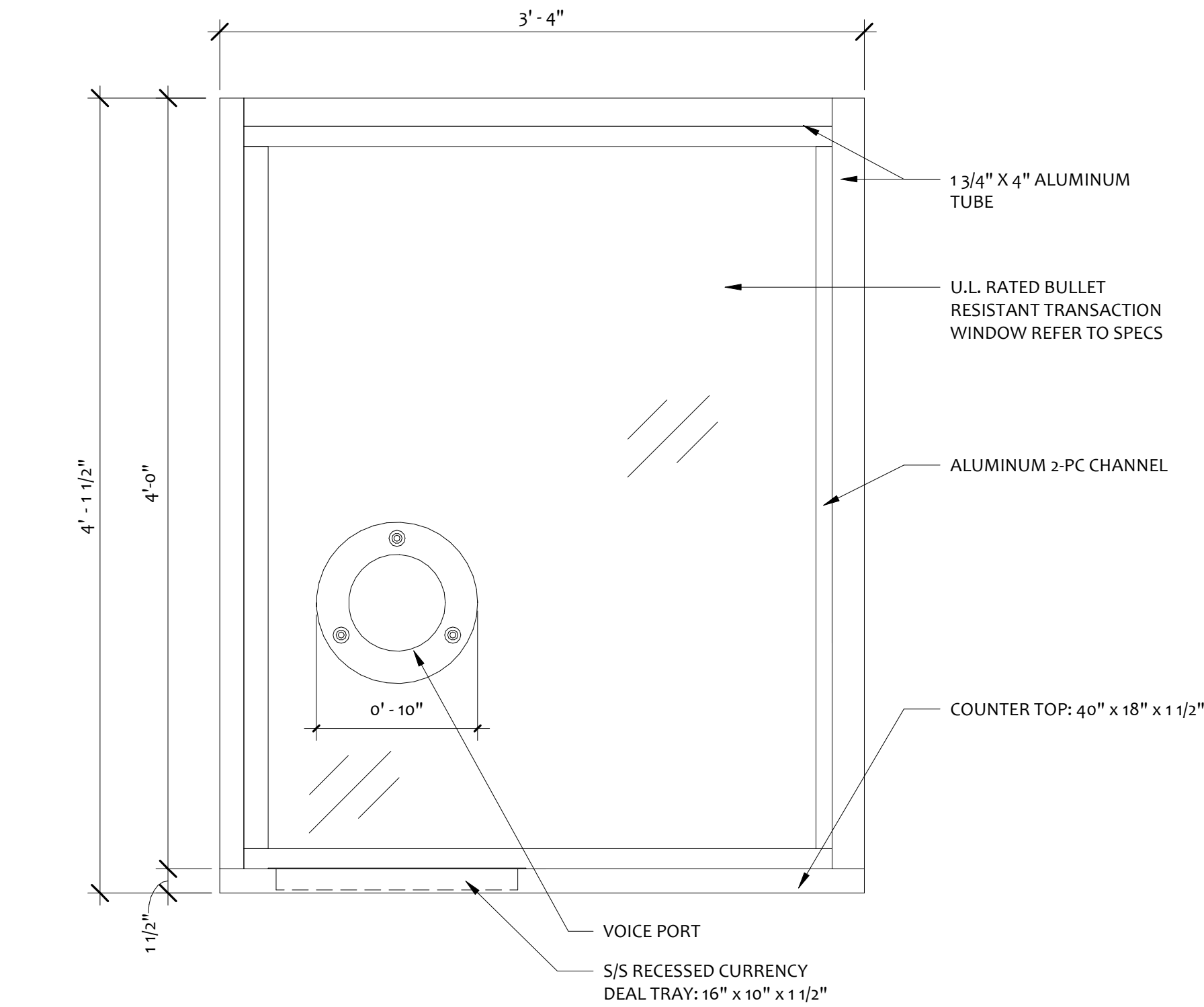
4 SECURE TRANSACTION WINDOW ELEVATION 1 1/2" = 1'-0"
