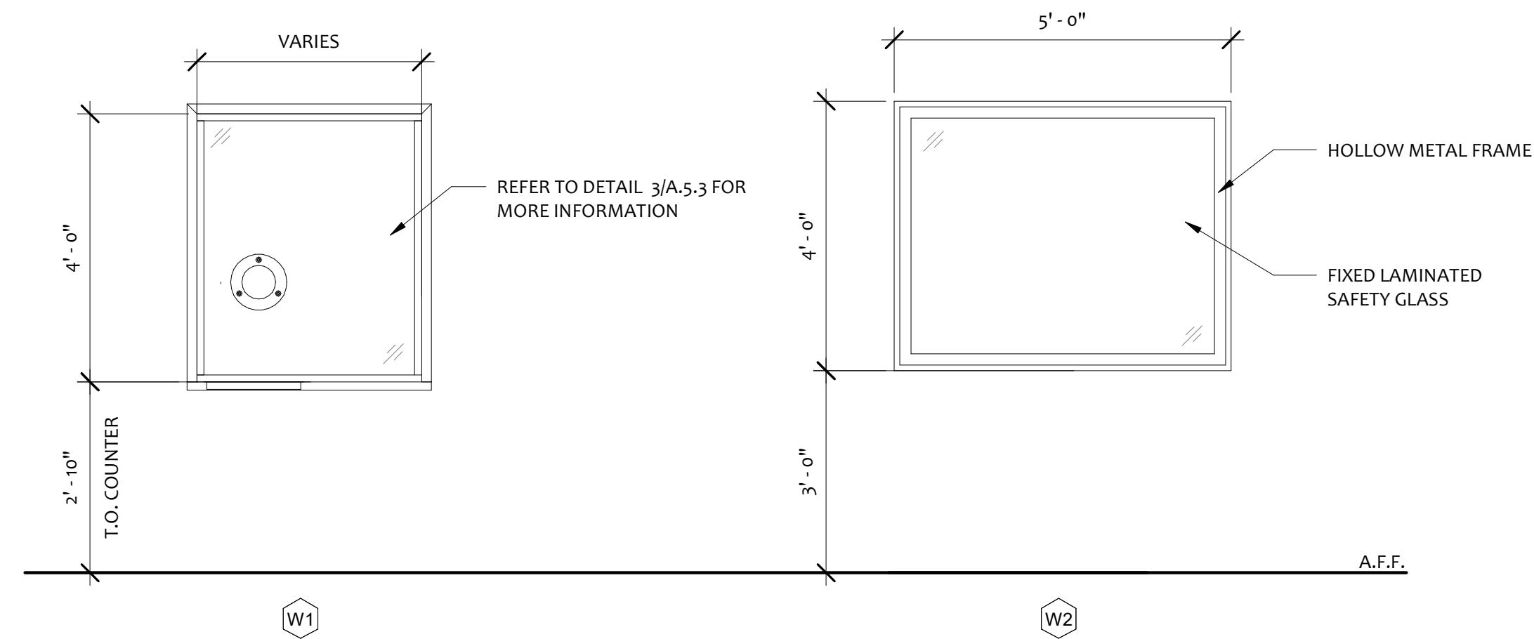
1 WINDOW ELEVATIONS 1/2" = 1'-0"
