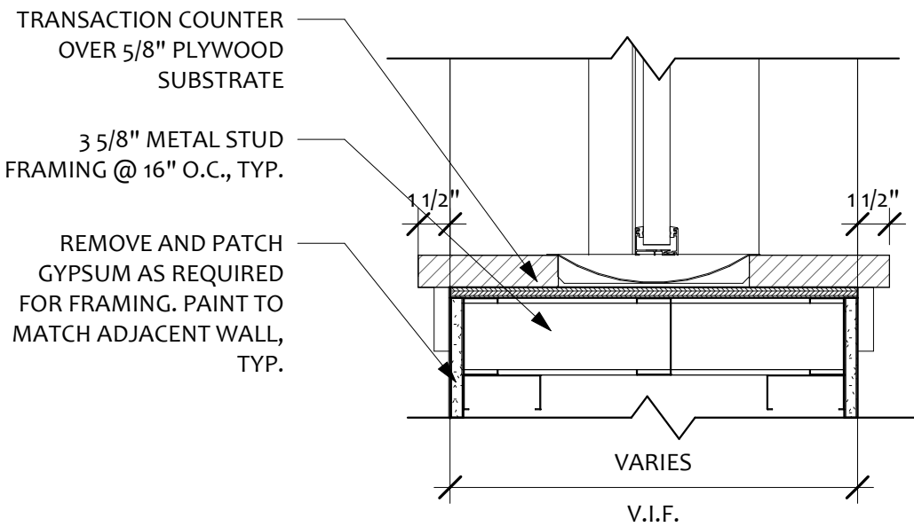
6 SECURE TRANSACTION WINDOW SECTION IN EXISTING WALL 1 1/2" = 1'-0"
