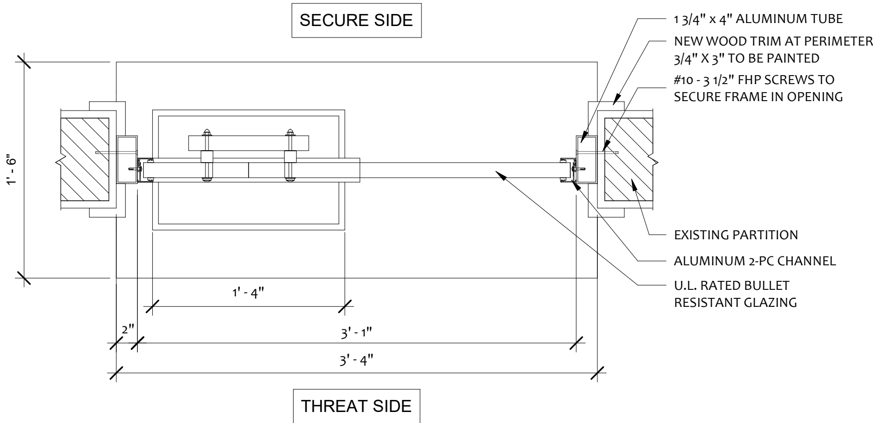
2 SECURE TRANSACTION WINDOW PLAN DETAIL 1 1/2" = 1'-0"
