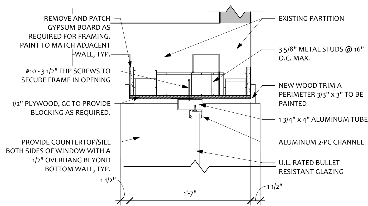
3 CONSTRUCTION PLAN - THIRD FLOOR - Callout 2 1 1/2" = 1'-0"
