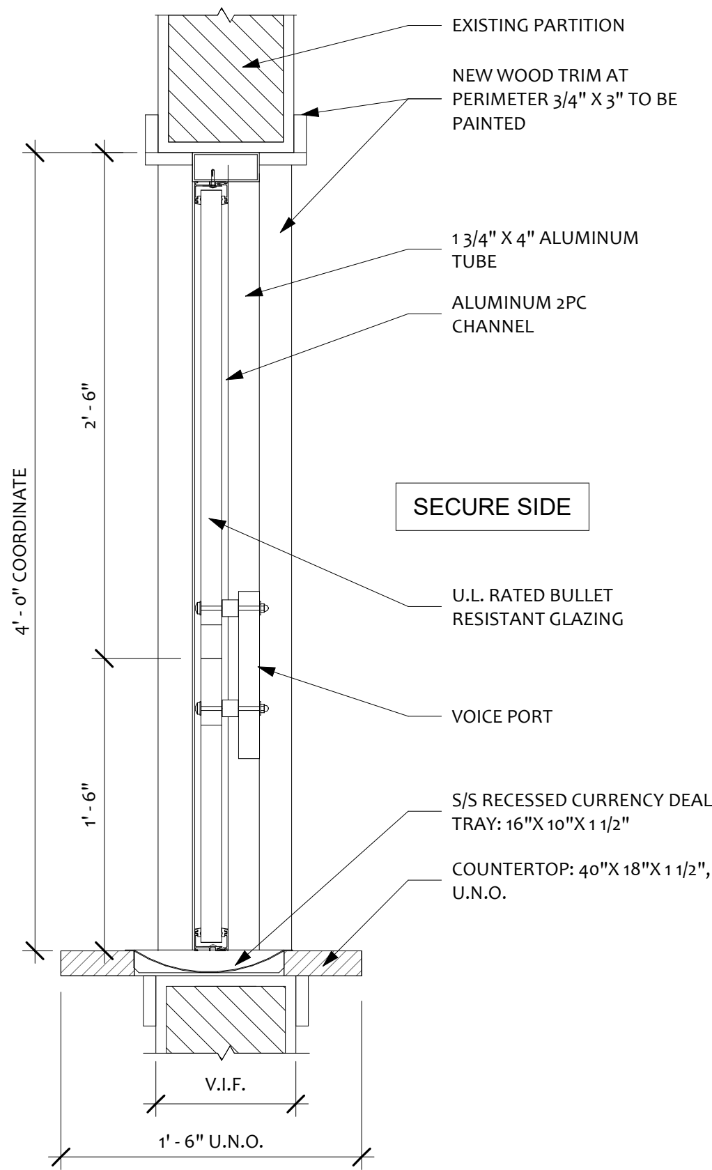
5 SECURE TRANSACTION WINDOW SECTION 1 1/2" = 1'-0"
